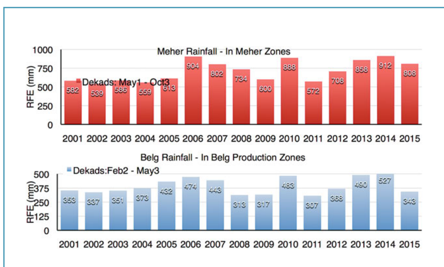
Figure 6: Belg and Meher Rainfall Amounts (mm)
